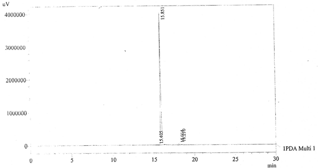
Chromatogram 2',3'-Dimethoxyflavone D:\promonence\Data\2013\July-2013\110713G.lcd
